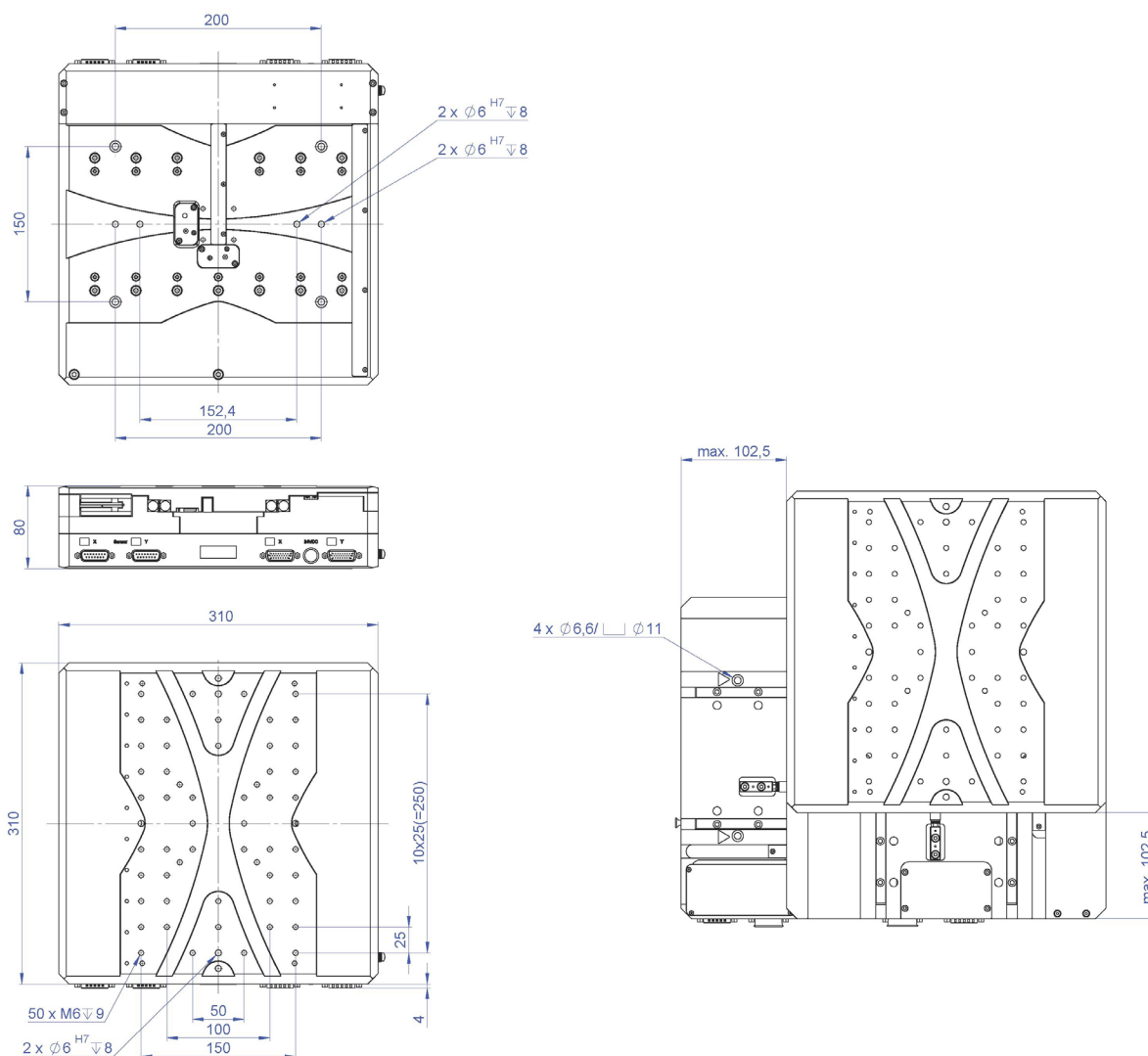
V-731, dimensions in mm
