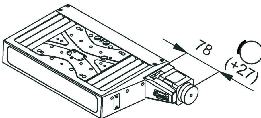
HPS-170, stepper motor, dimensions in mm. Note that a comma is used in the drawings instead of a decimal point.
