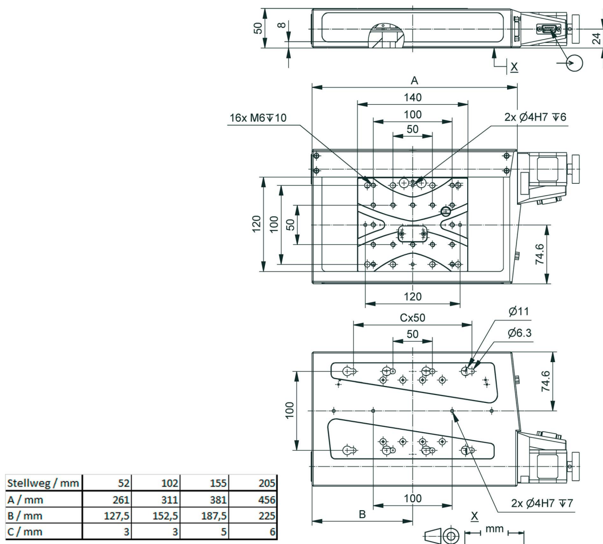
HPS-170, dimensions in mm. Note that a comma is used in the drawings instead of a decimal point.
