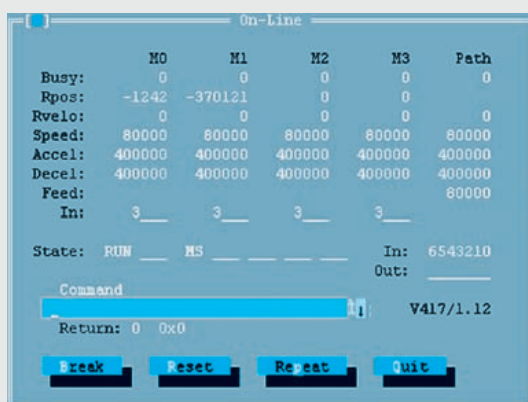
MotionBasic™ compiler
